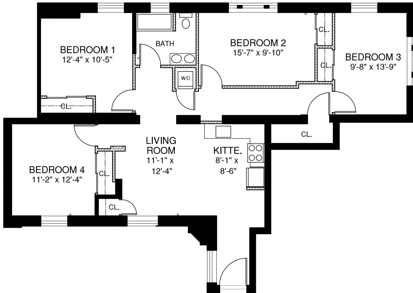
PROPOSED FLOOR PLAN Scale: 1/8" = 1'-0"
